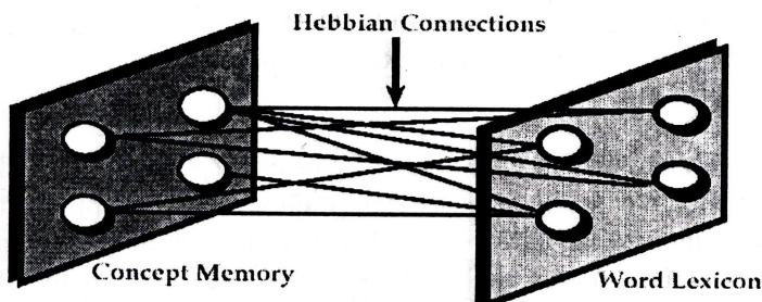
Fig. 4: Naming connections between the Concept Memory and the Word Lexicon.
